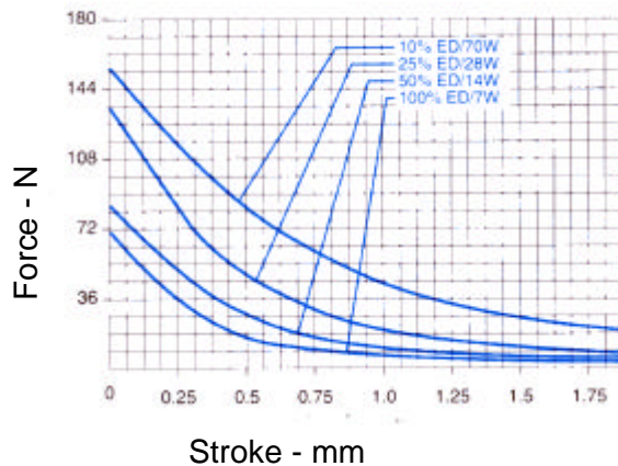
Typical Force @20°C 2EFM
