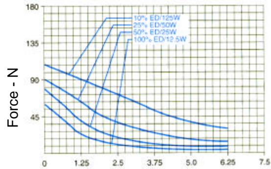
Typical Speed @ 20°C 4ECM
