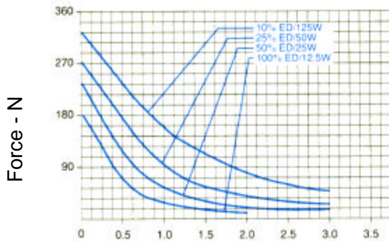
Typical Force @20°C 4EFM
