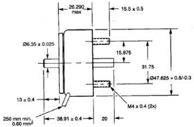
Shown Energised
