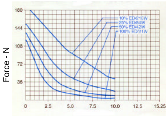
Stroke - mm
