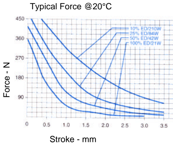
5SFM Short Stroke, Flat Face Part No. : 282349-0XX
