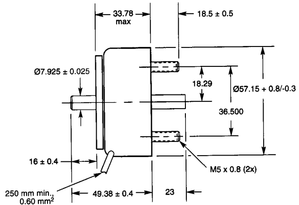
Shown Energised
