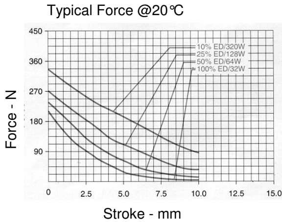
6ECM Medium Stroke, Conical Face Part No. : 282352-0XX
