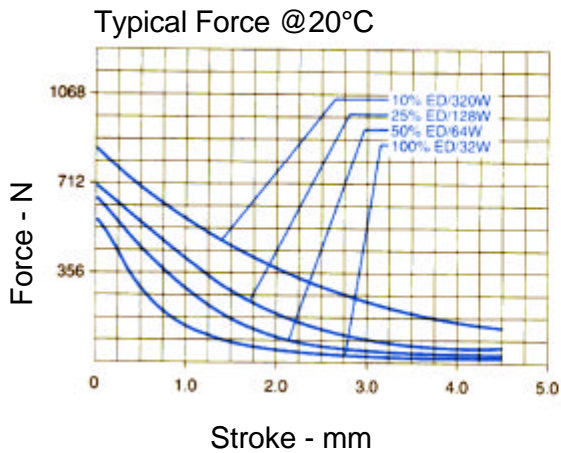
6SFM Short Stroke, Flat Face Part No. : 282351-0XX
