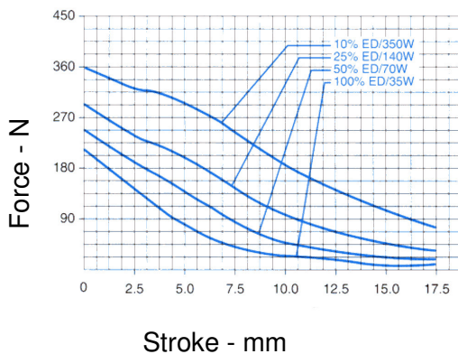
Typical Force @20°C
