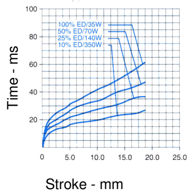
Typical Speed @ No Load, 20°C
