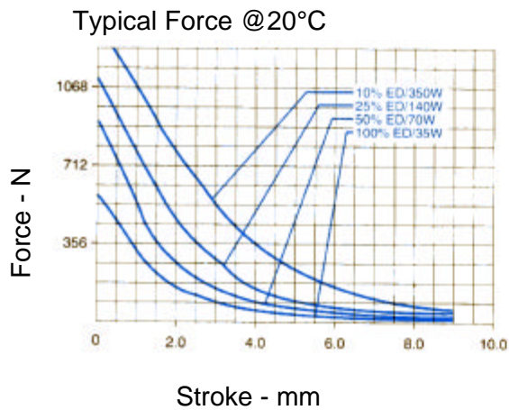
7SFM Short Stroke, Flat Face Part No. : 282353-0XX
